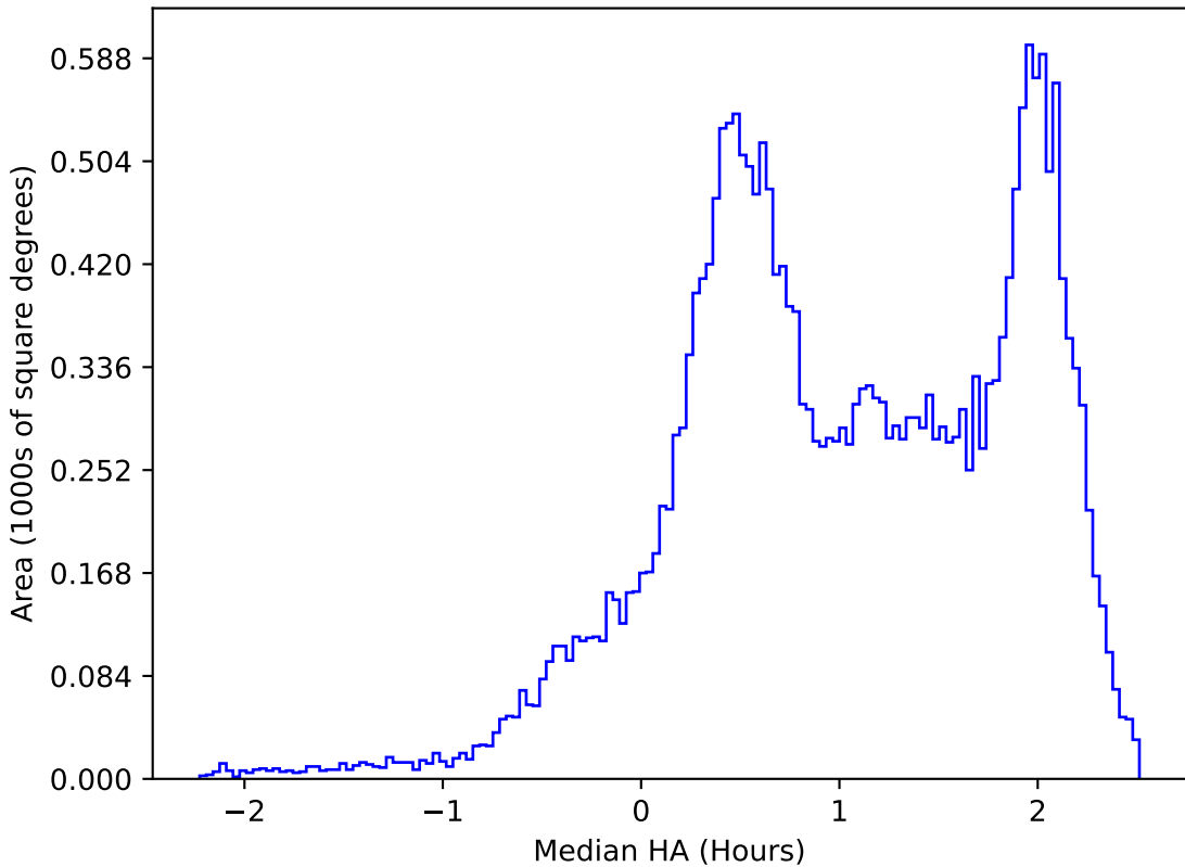
ddf_acor_sf15_lsf40_lsr10_v3.4_10yrs All sky z band: Median HA
