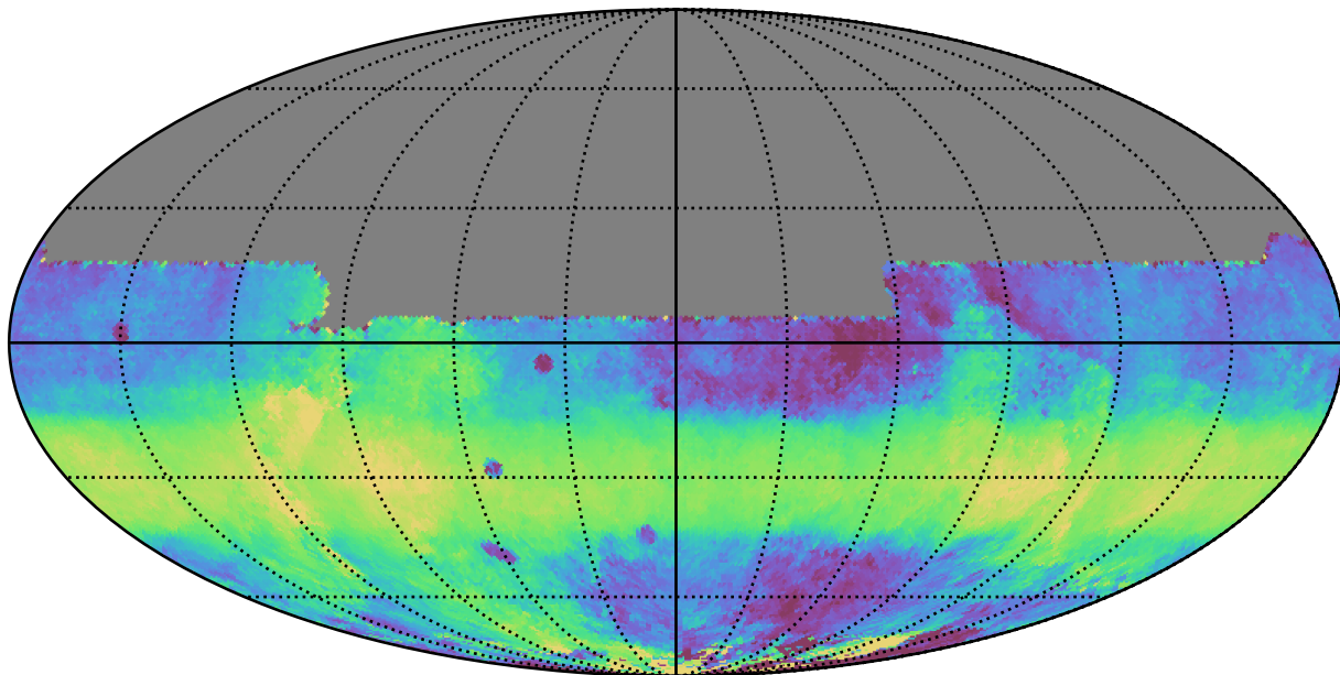
ddf_acor_sf15_lsf40_lsr10_v3.4_10yrs All sky y band: Median HA
