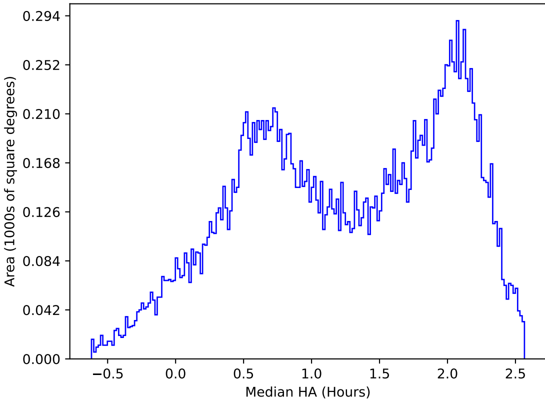
ddf_acor_sf15_ls40_lsr10_v3.4_10yrs All sky y band: Median HA
