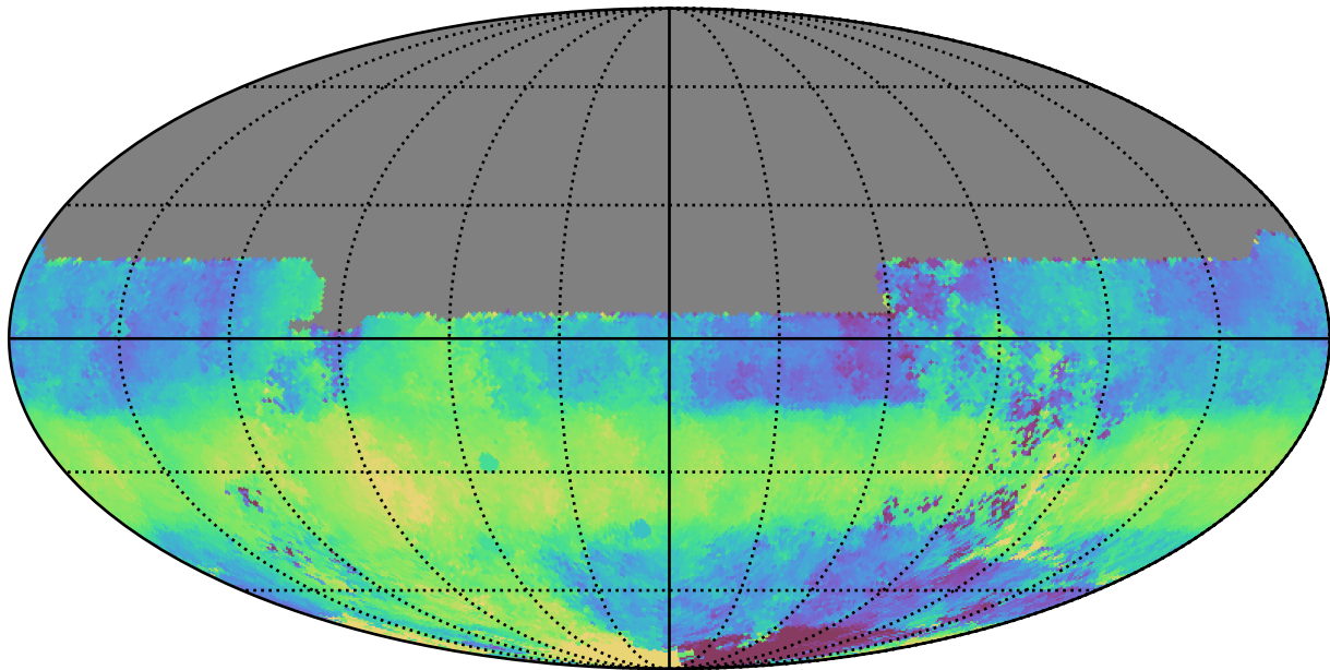
ddf_acor_sf15_lsf40_lsr10_v3.4_10yrs All sky u band: Median HA
