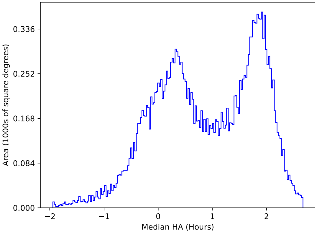
ddf_acor_sf15_lsf40_lsr10_v3.4_10yrs All sky u band: Median HA
