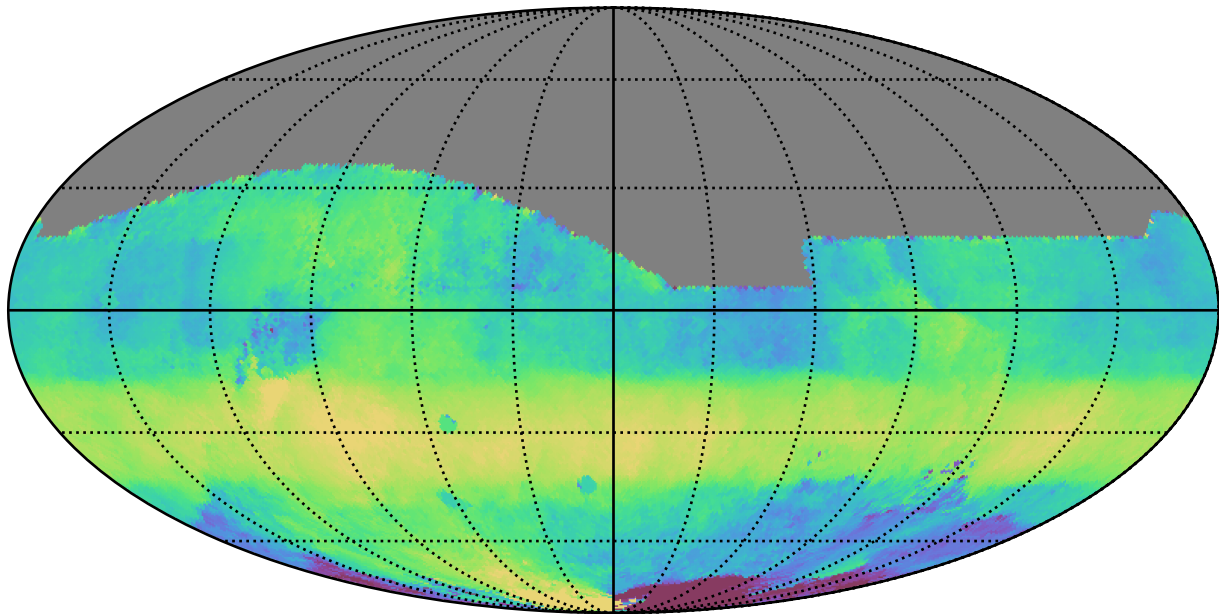
ddf_acor_sf15_lsf40_lsr10_v3.4_10yrs All sky r band: Median HA
