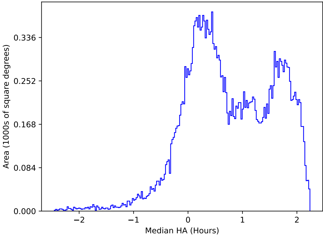
ddf_acor_sf15_lsf40_lsr10_v3.4_10yrs All sky r band: Median HA
