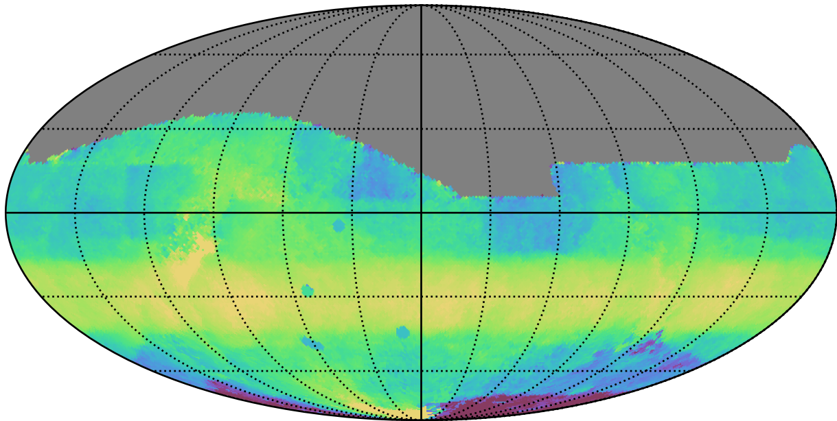
ddf_acor_sf15_lsf40_lsr10_v3.4_10yrs All sky i band: Median HA
