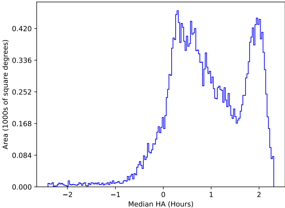
ddf_acor_sf15_lsf40_lsr10_v3.4_10yrs All sky i band: Median HA
