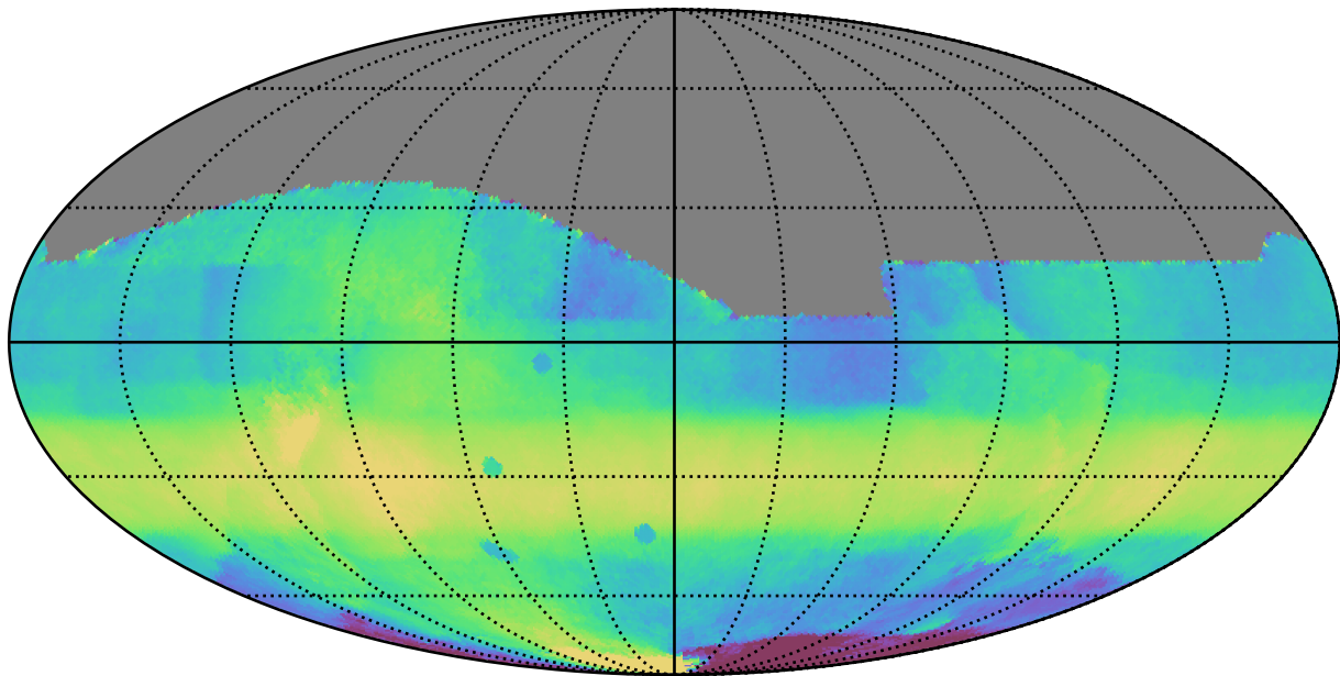
ddf_acor_sf15_lsf40_lsr10_v3.4_10yrs All sky all bands: Median HA
