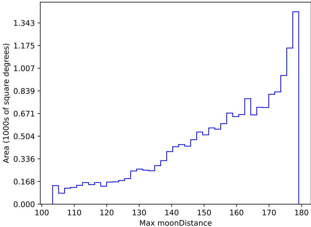
ddf_acor_sf15_lsf40_lsr10_v3.4_10yrs WFD i band: Max moonDistance
