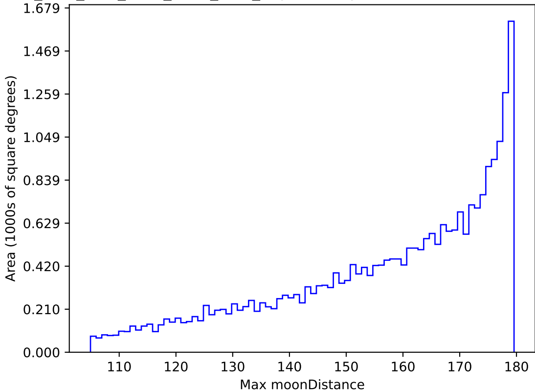
ddf_acor_sf15_lsf40_lsr10_v3.4_10yrs All sky all bands: Max moonDistance
