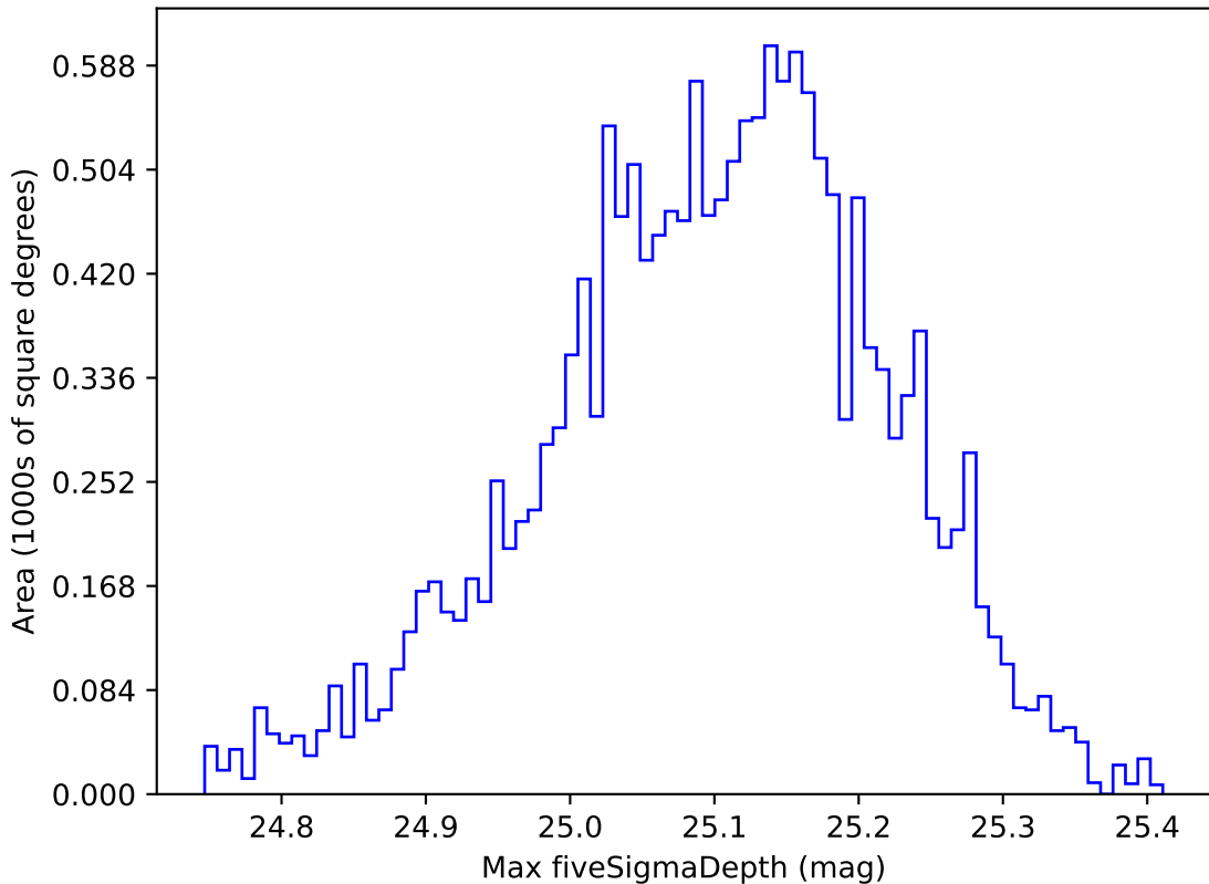
ddf_acor_sf15_lsf40_lsr10_v3.4_10yrs WFD all bands: Max fiveSigmaDepth
