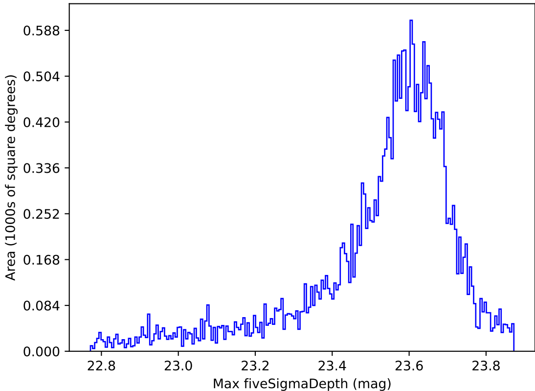
ddf_acor_sf15_ls40_lsr10_v3.4_10yrs All sky z band: Max fiveSigmaDepth
