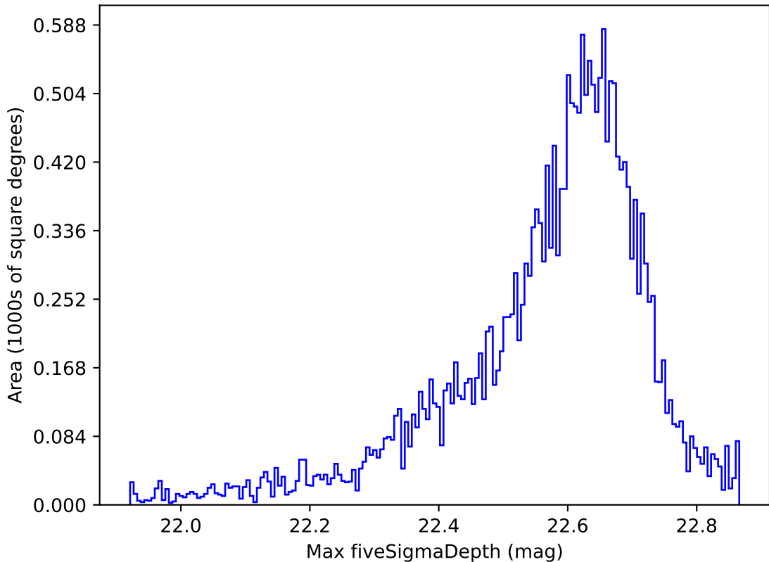
ddf_acor_sf15_ls40_lsr10_v3.4_10yrs All sky y band: Max fiveSigmaDepth
