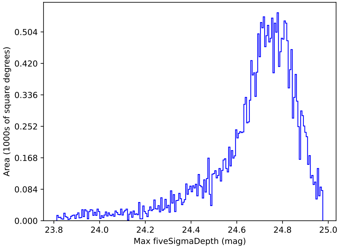
ddf_acor_sf15_lsf40_lsr10_v3.4_10yrs All sky r band: Max fiveSigmaDepth
