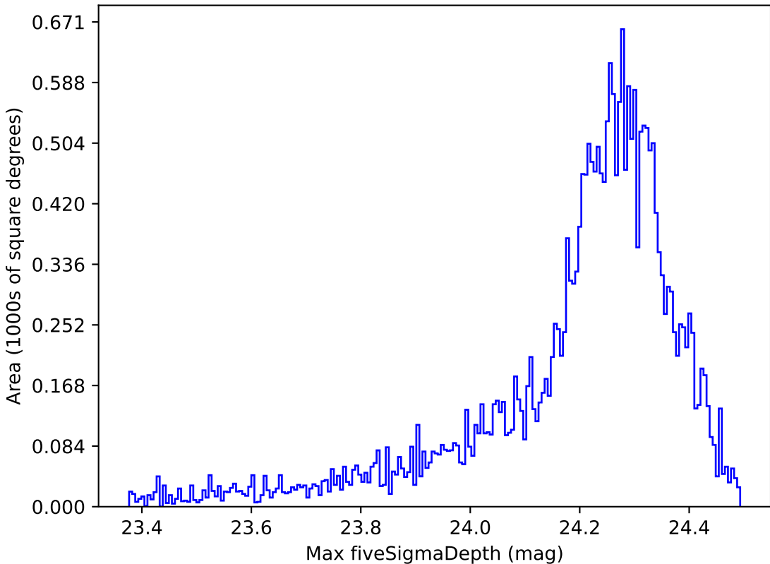
ddf_acor_sf15_lsf40_lsr10_v3.4_10yrs All sky i band: Max fiveSigmaDepth
