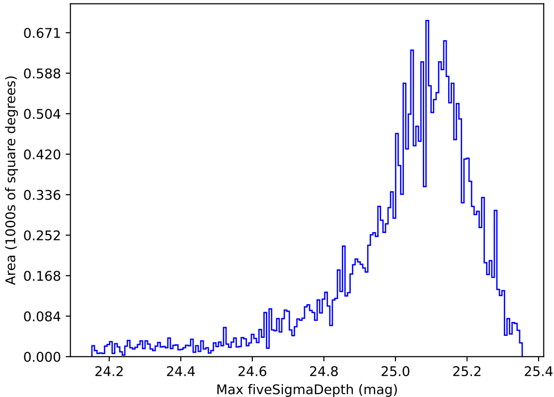
ddf_acor_sf15_lsf40_lsr10_v3.4_10yrs All sky g band: Max fiveSigmaDepth
