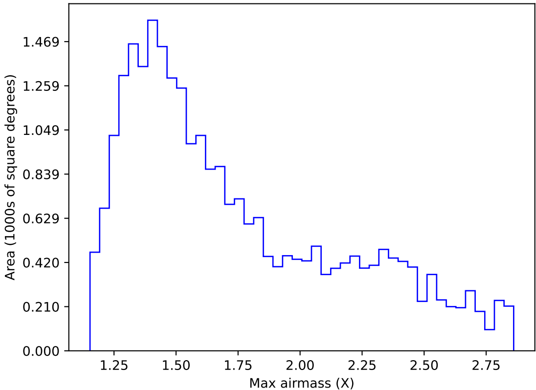
ddf_acor_sf15_lsf40_lsr10_v3.4_10yrs Yr 1 z band: Max airmass
