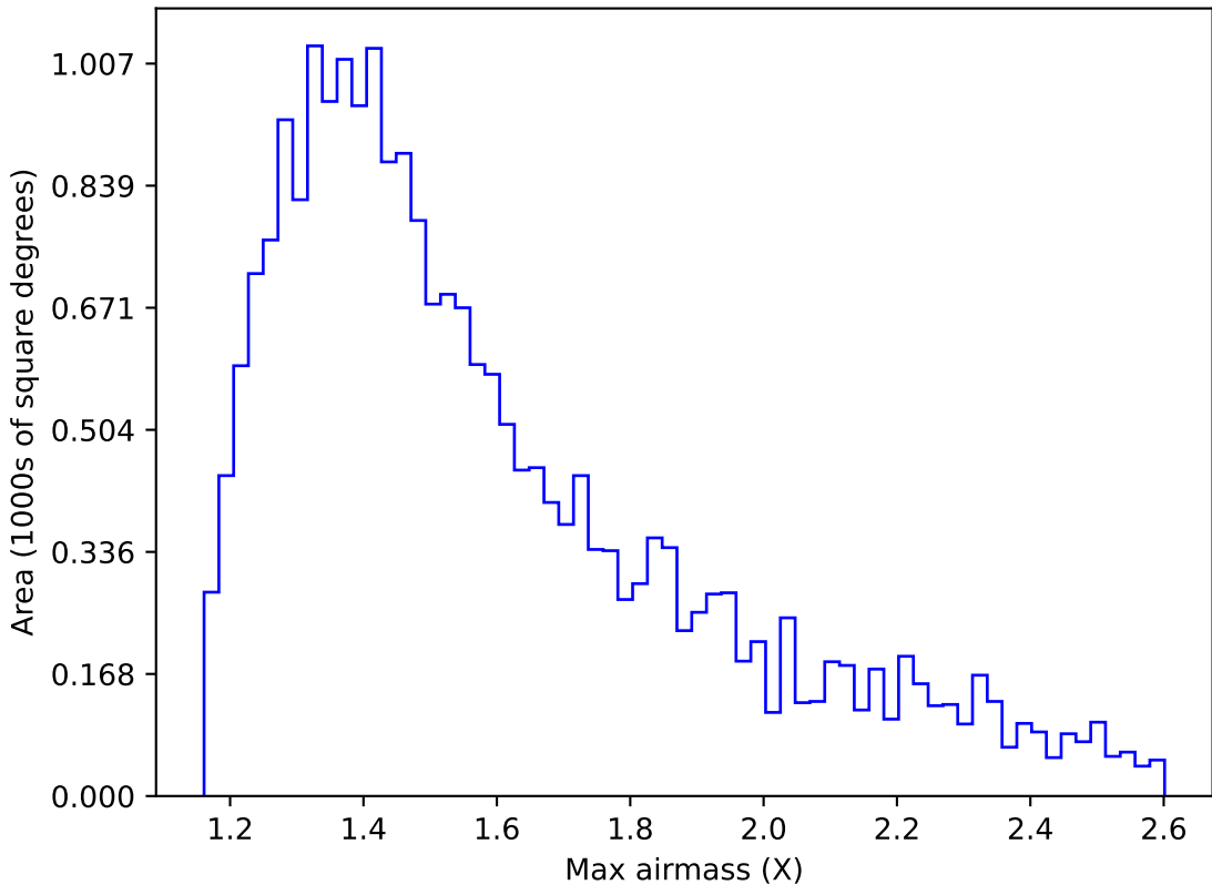
ddf_acor_sf15_lsf40_lsr10_v3.4_10yrs Yr 1 y band: Max airmass
