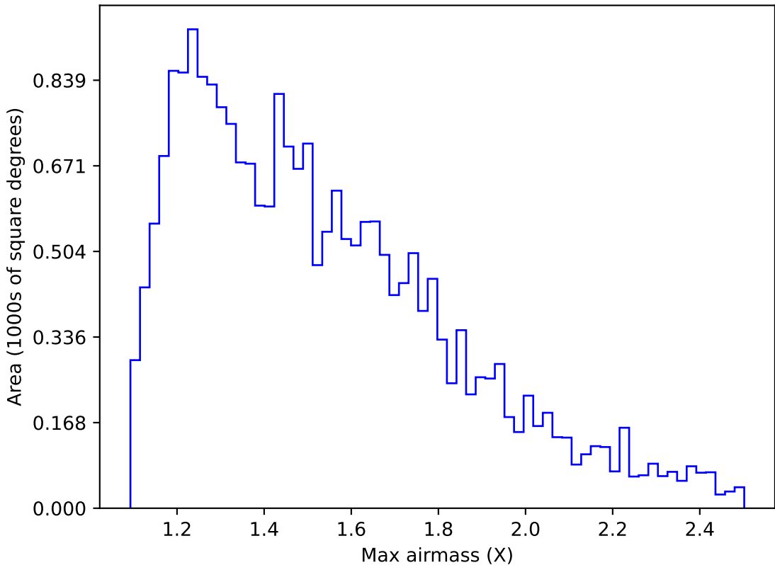
ddf_acor_sf15_lsf40_lsr10_v3.4_10yrs Yr 1 u band: Max airmass
