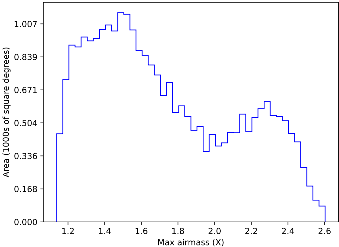
ddf_acor_sf15_lsf40_lsr10_v3.4_10yrs Yr 1 r band: Max airmass
