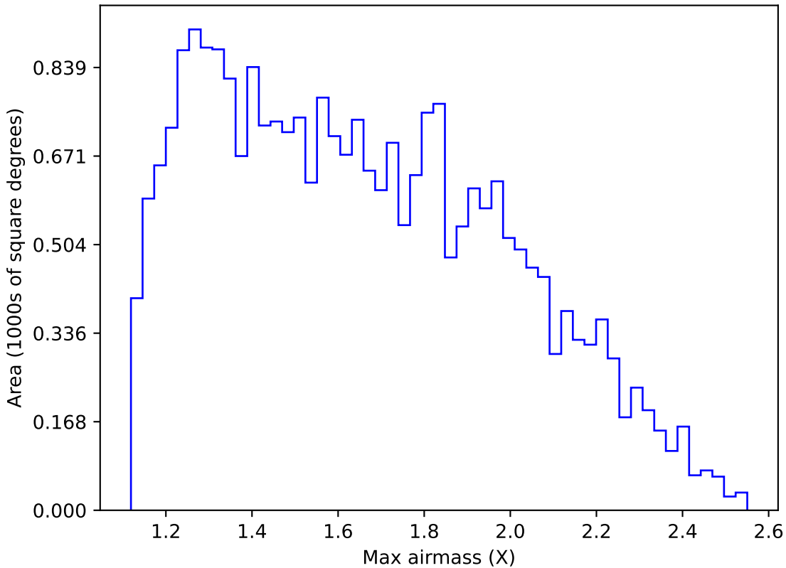
ddf_acor_sf15_lsf40_lsr10_v3.4_10yrs Yr 1 g band: Max airmass
