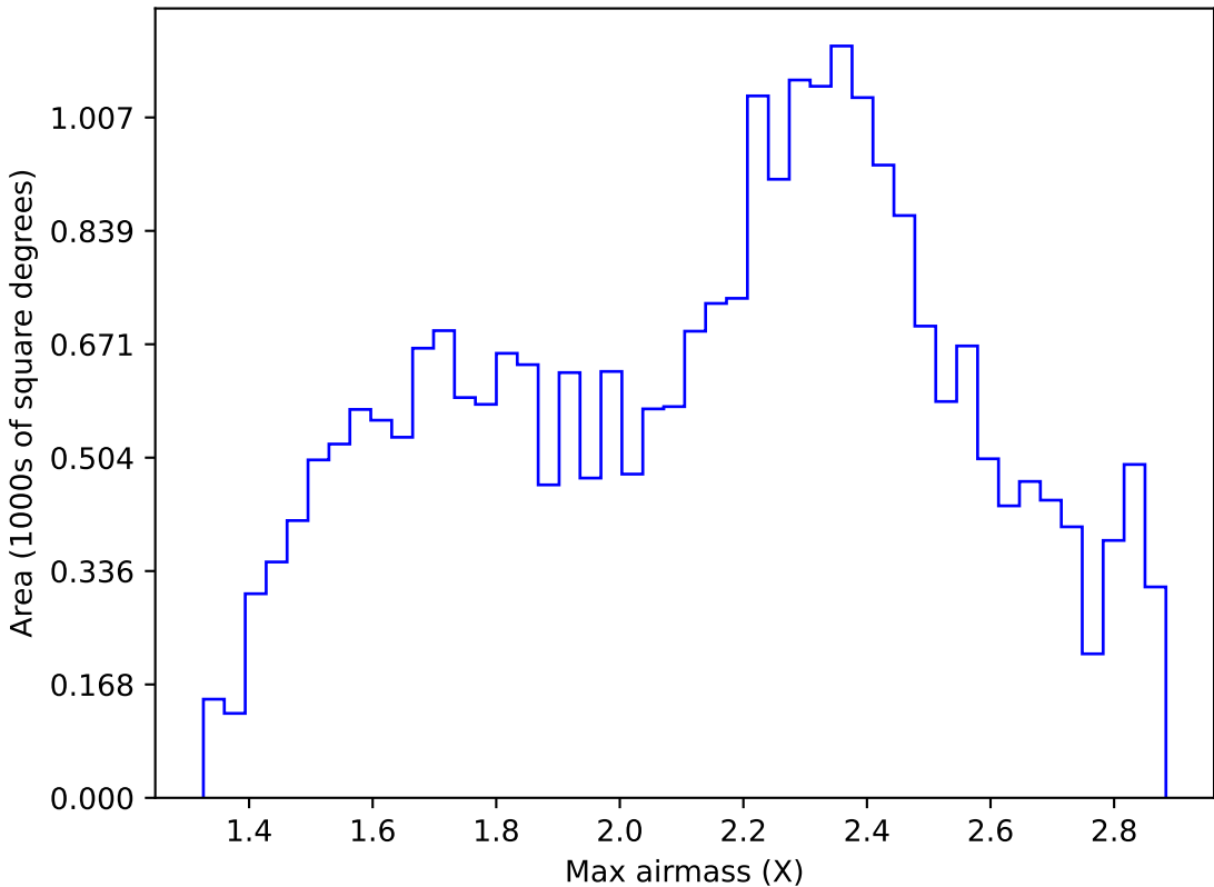
ddf_acor_sf15_lsf40_lsr10_v3.4_10yrs Yr 1 all bands: Max airmass
