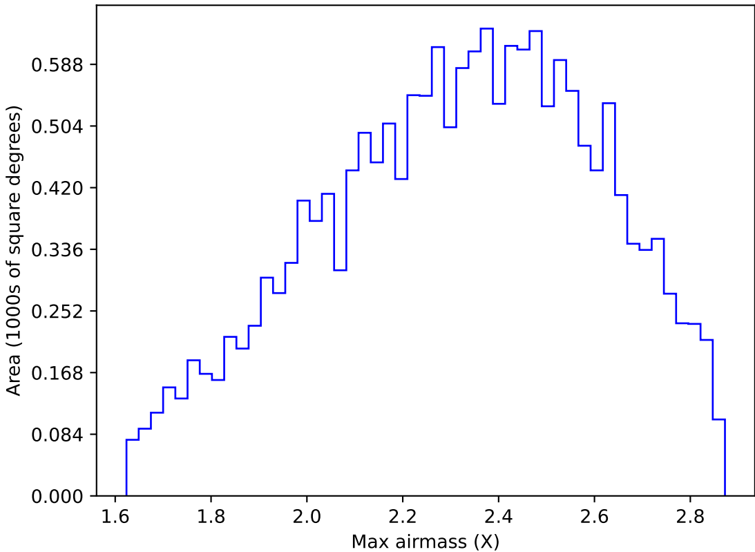
ddf_acor_sf15_lsf40_lsr10_v3.4_10yrs WFD y band: Max airmass
