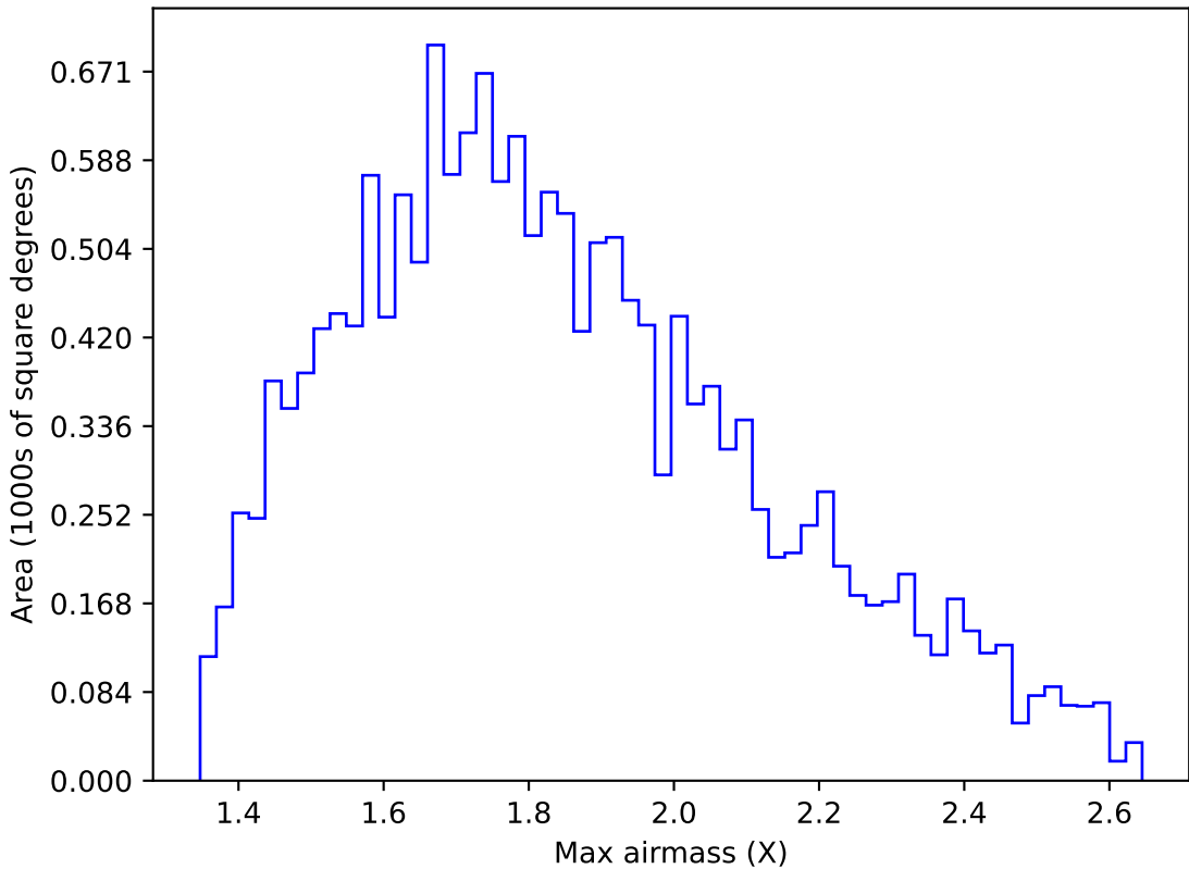
ddf_acor_sf15_ls40_lsr10_v3.4_10yrs WFD u band: Max airmass
