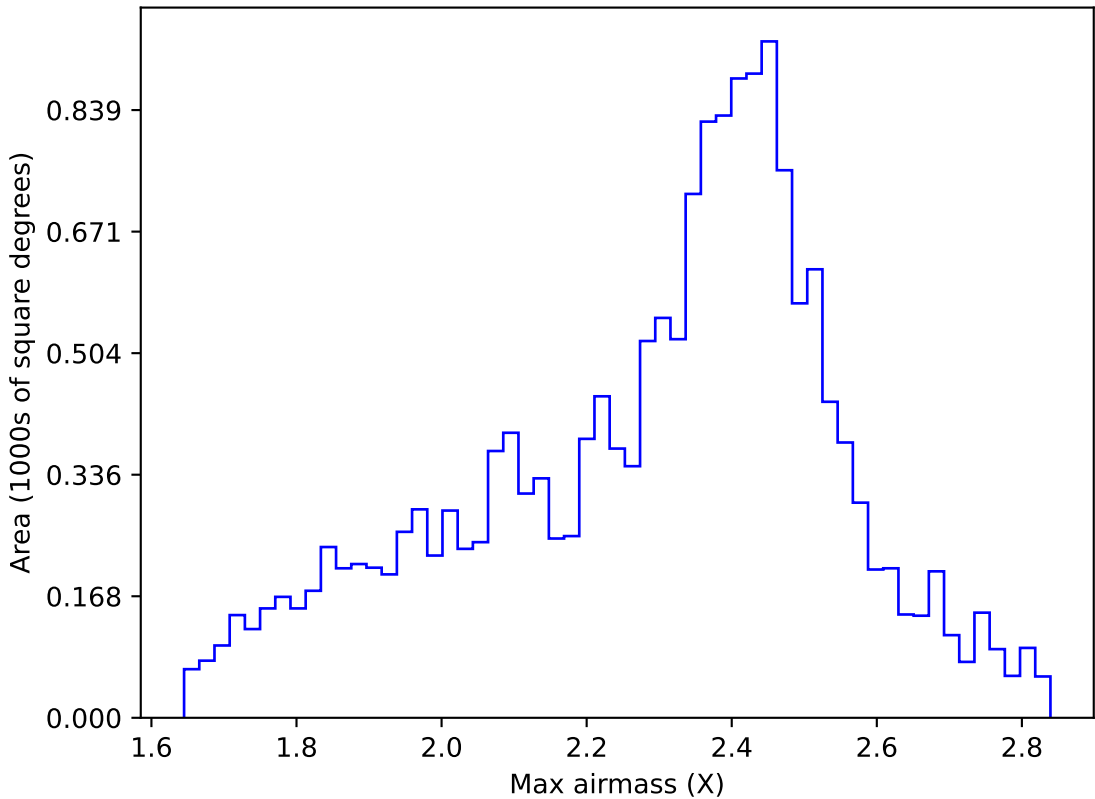
ddf_acor_sf15_lsf40_lsr10_v3.4_10yrs WFD r band: Max airmass
