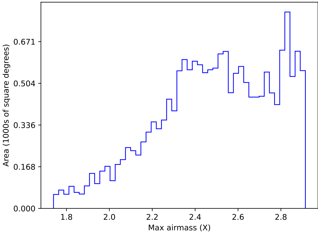
ddf_acor_sf15_lsf40_lsr10_v3.4_10yrs WFD i band: Max airmass
