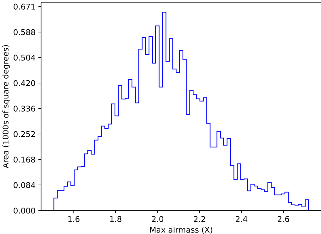
ddf_acor_sf15_lsf40_lsr10_v3.4_10yrs WFD g band: Max airmass
