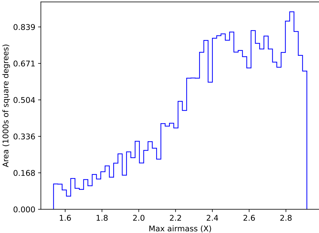
ddf_acor_sf15_lsf40_lsr10_v3.4_10yrs All sky z band: Max airmass
