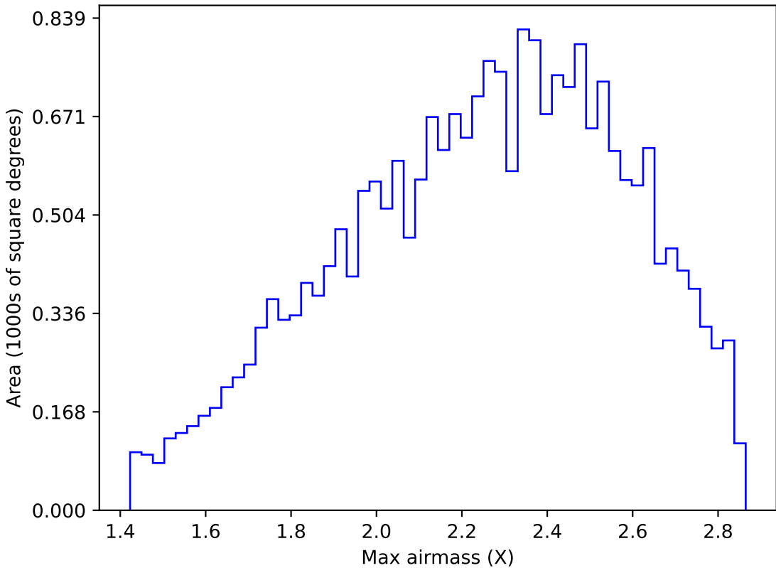
ddf_acor_sf15_lsf40_lsr10_v3.4_10yrs All sky y band: Max airmass
