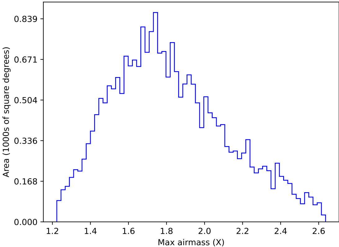
ddf_acor_sf15_lsf40_lsr10_v3.4_10yrs All sky u band: Max airmass
