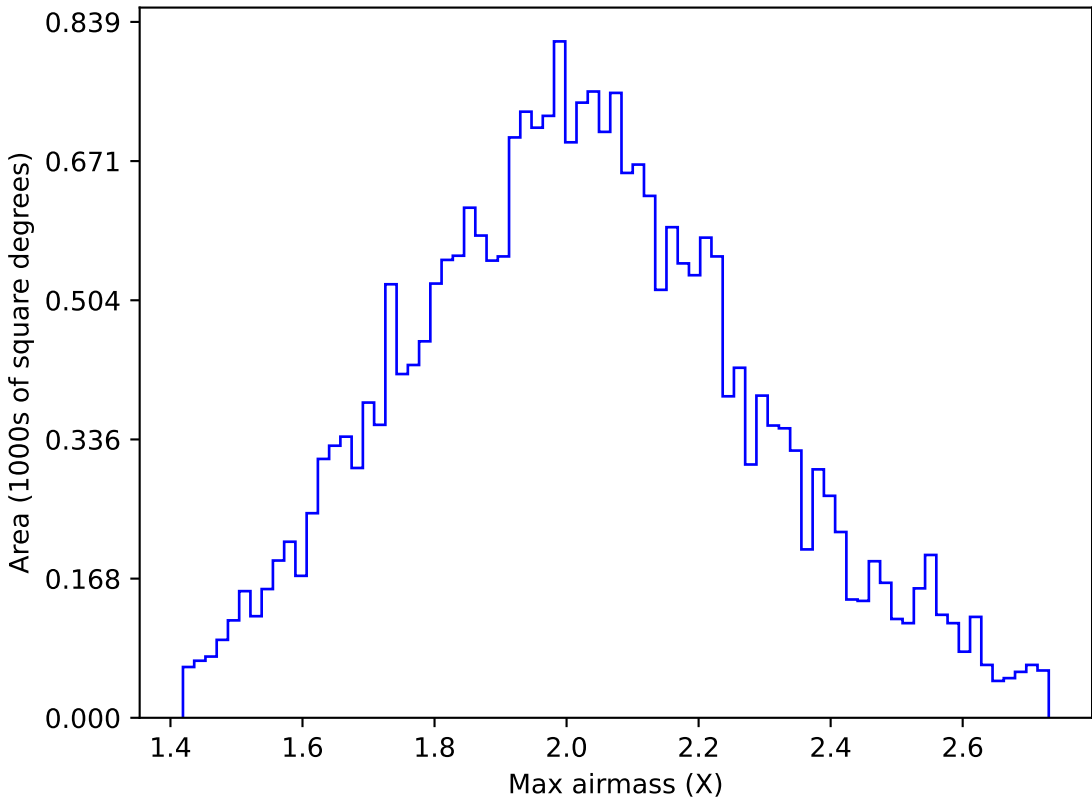
ddf_acor_sf15_lsf40_lsr10_v3.4_10yrs All sky g band: Max airmass
