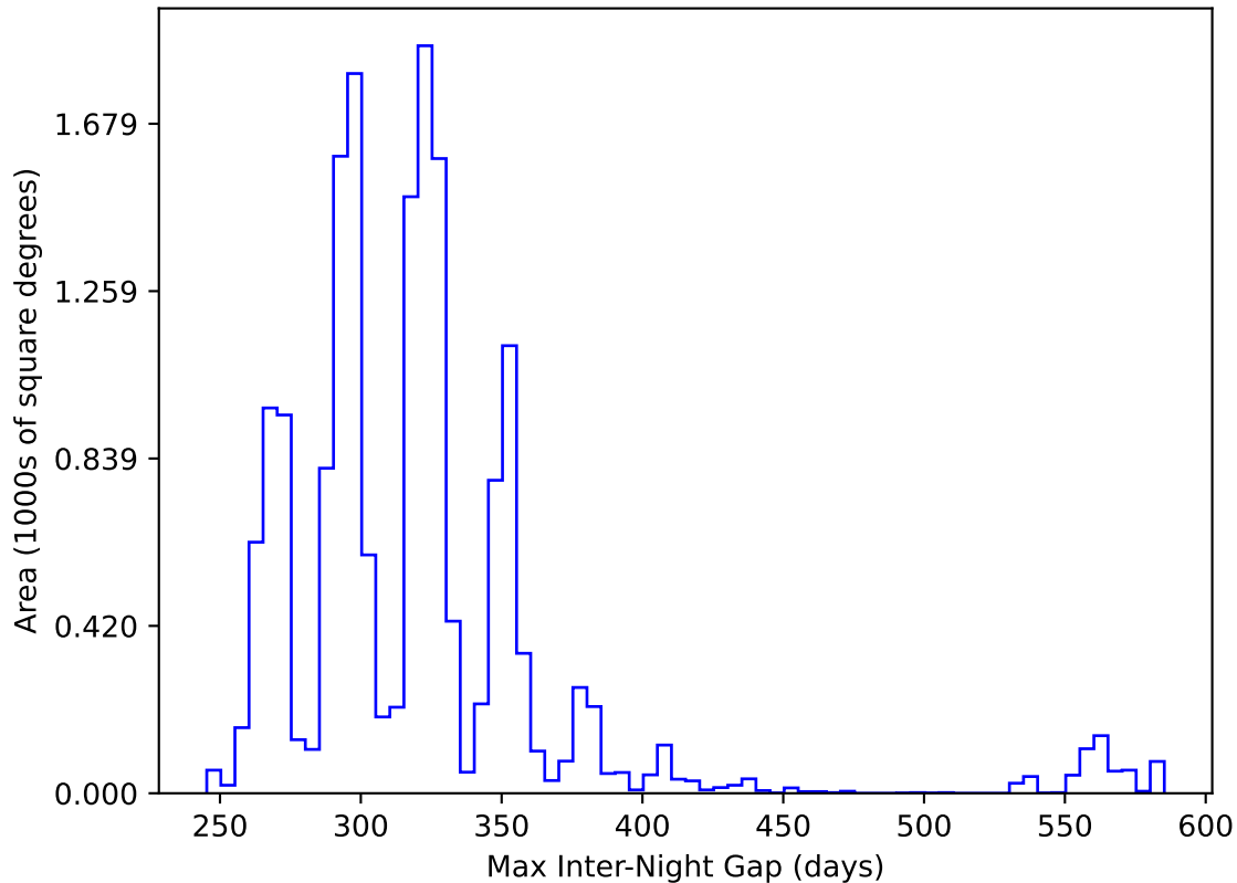
ddf_acor_sf15_lsf40_lsr10_v3.4_10yrs WFD y band: Max Inter-Night Gap
