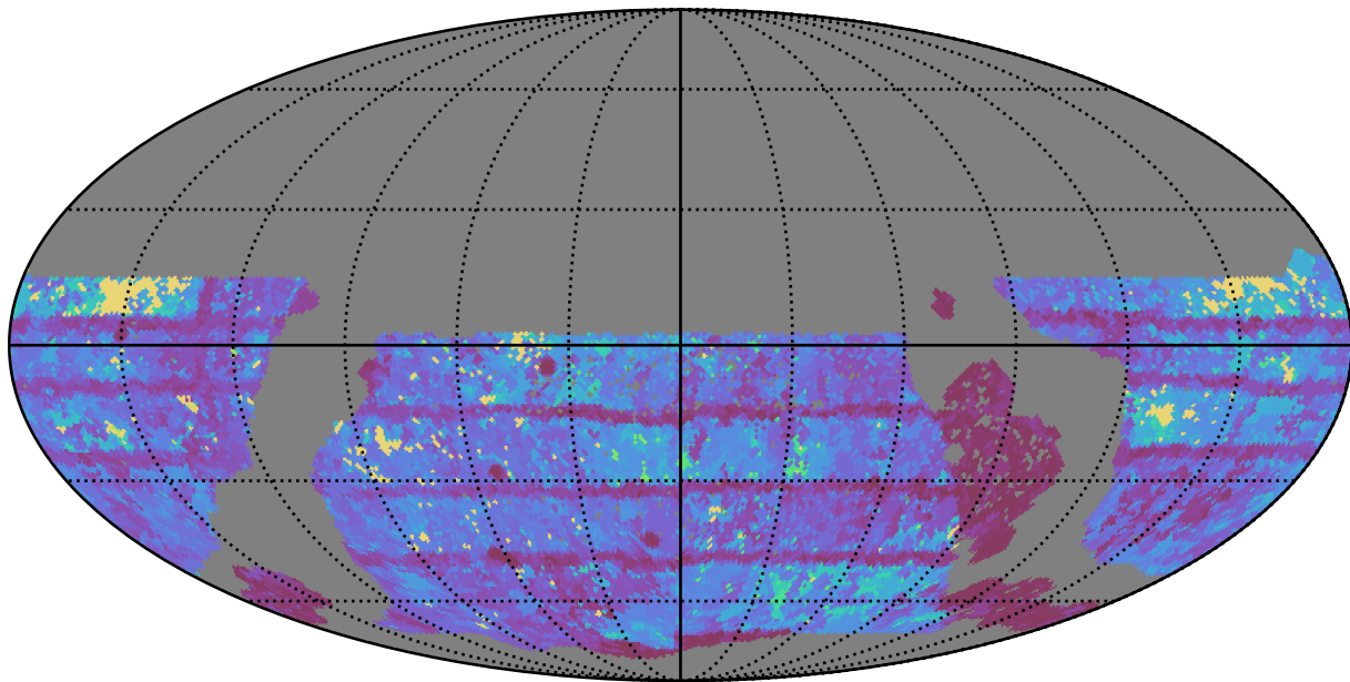
ddf_acor_sf15_lsf40_lsr10_v3.4_10yrs WFD r band: Max Inter-Night Gap
