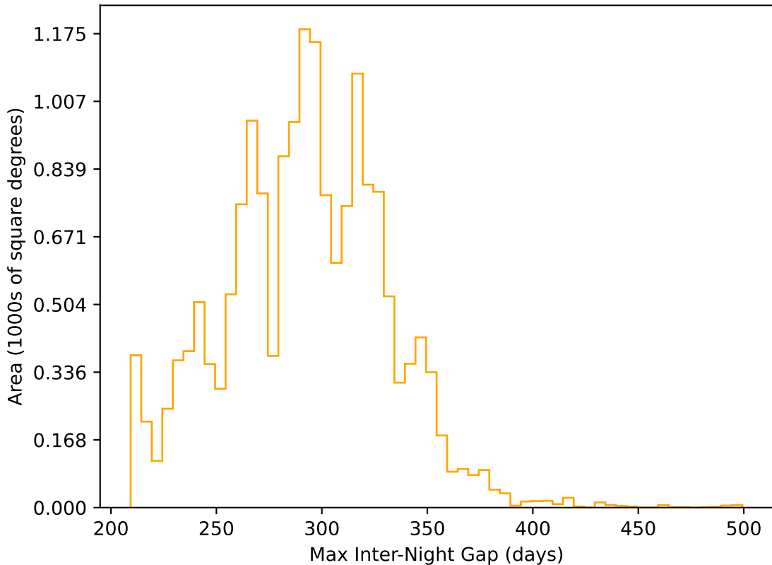
ddf_acor_sf15_lsf40_lsr10_v3.4_10yrs WFD r band: Max Inter-Night Gap
