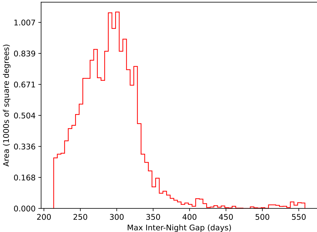
ddf_acor_sf15_lsf40_lsr10_v3.4_10yrs WFD i band: Max Inter-Night Gap
