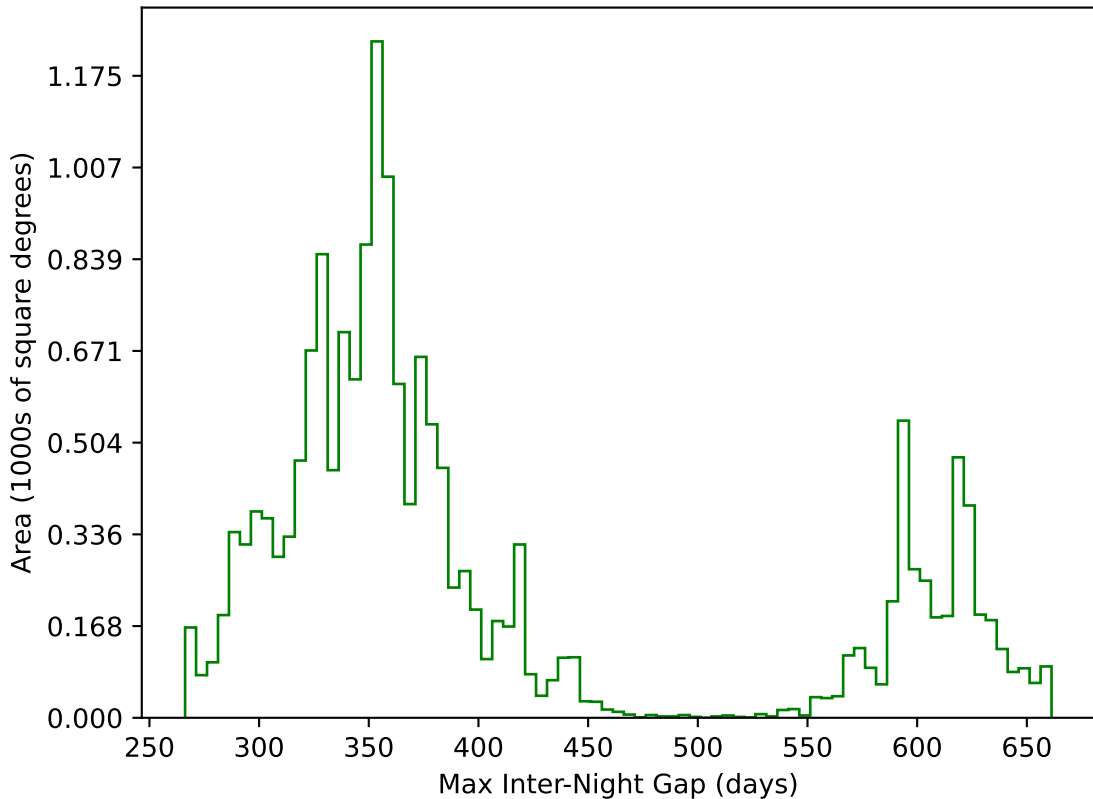
ddf_acor_sf15_lsf40_lsr10_v3.4_10yrs WFD g band: Max Inter-Night Gap
