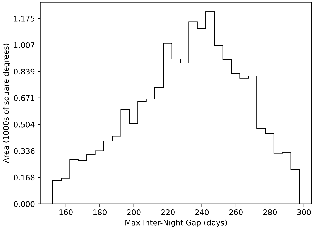
ddf_acor_sf15_lsf40_lsr10_v3.4_10yrs WFD all bands: Max Inter-Night Gap
