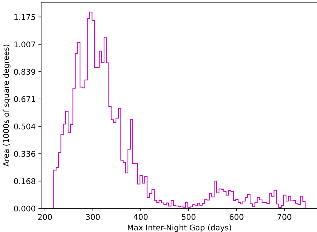
ddf_acor_sf15_lsf40_lsr10_v3.4_10yrs All sky z band: Max Inter-Night Gap
