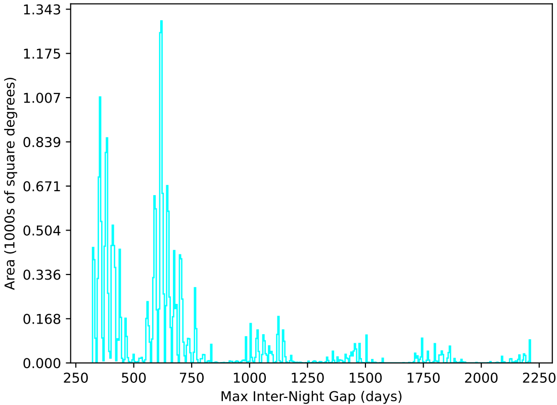
ddf_acor_sf15_lsf40_lsr10_v3.4_10yrs All sky u band: Max Inter-Night Gap
