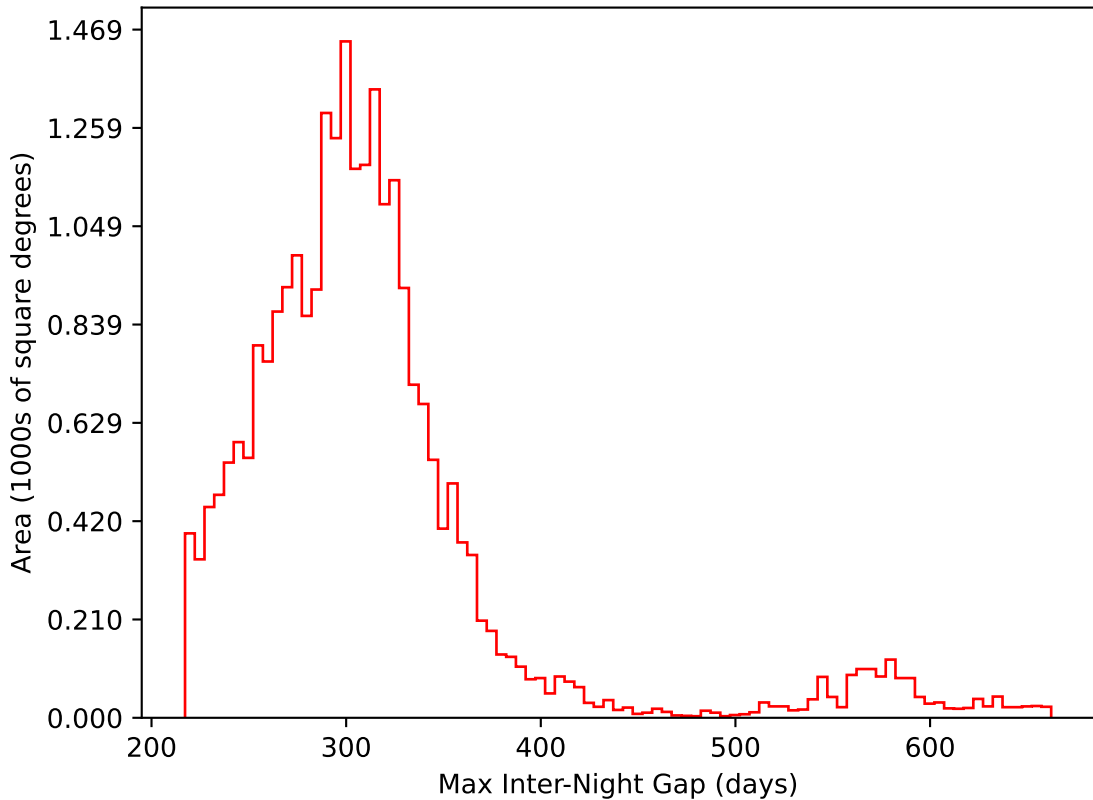
ddf_acor_sf15_lsf40_lsr10_v3.4_10yrs All sky i band: Max Inter-Night Gap
