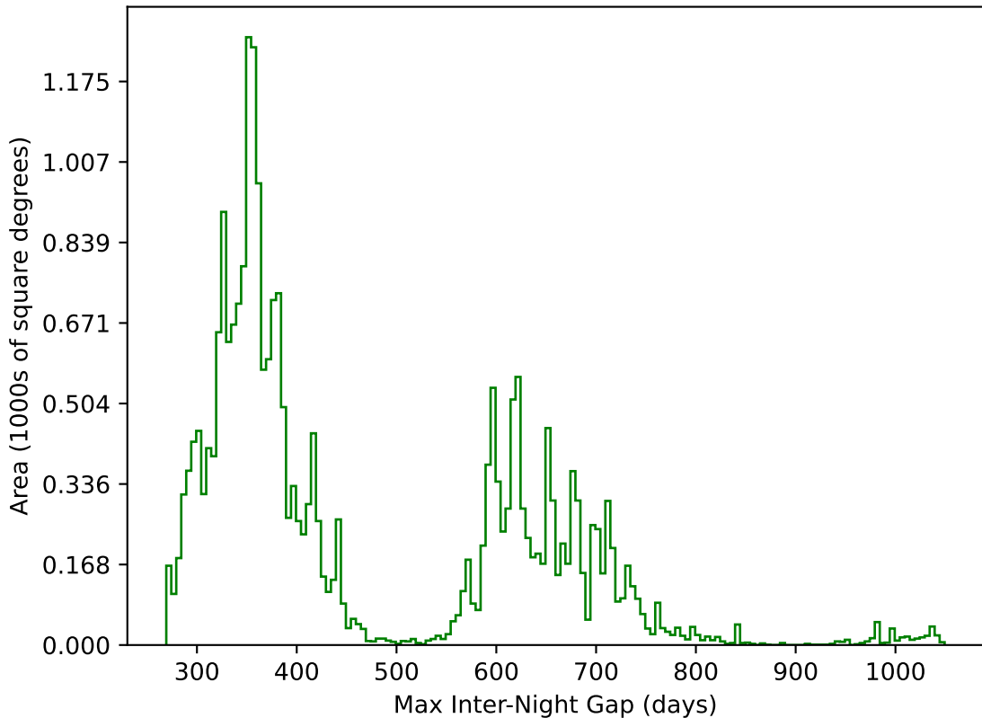
ddf_acor_sf15_lsf40_lsr10_v3.4_10yrs All sky g band: Max Inter-Night Gap
