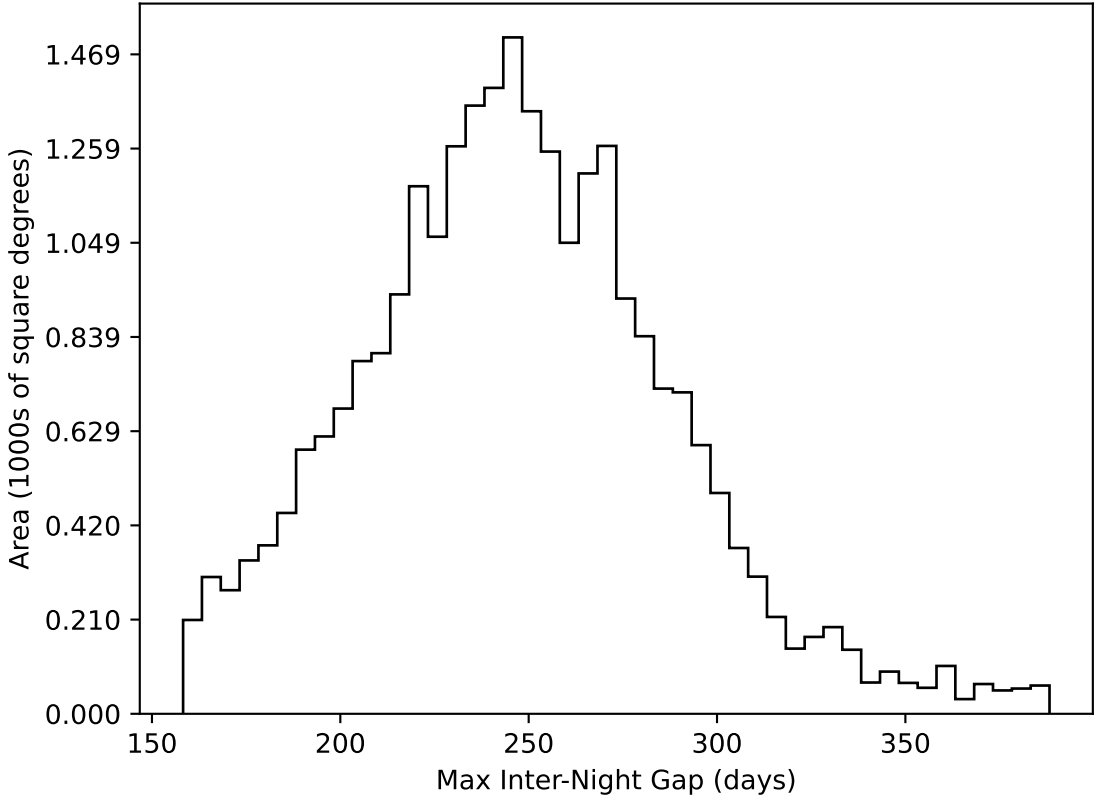
ddf_acor_sf15_lsf40_lsr10_v3.4_10yrs All sky all bands: Max Inter-Night Gap
