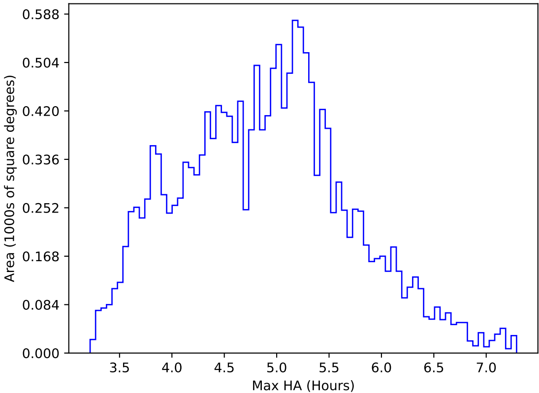
ddf_acor_sf15_lsf40_lsr10_v3.4_10yrs WFD z band: Max HA
