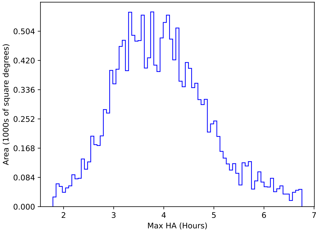
ddf_acor_sf15_lsf40_lsr10_v3.4_10yrs WFD u band: Max HA
