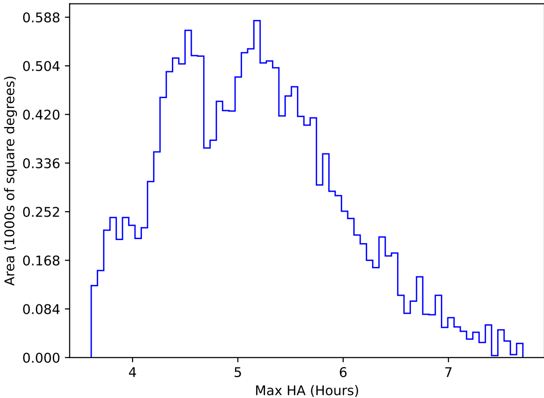
ddf_acor_sf15_lsf40_lsr10_v3.4_10yrs WFD all bands: Max HA
