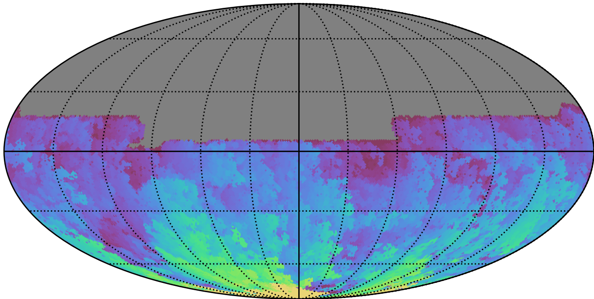
ddf_acor_sf15_lsf40_lsr10_v3.4_10yrs All sky u band: Max HA
