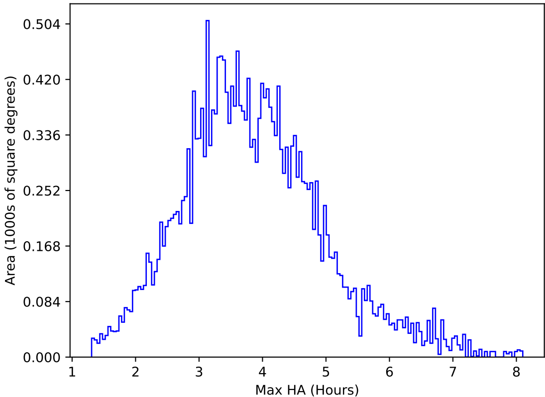
ddf_acor_sf15_lsf40_lsr10_v3.4_10yrs All sky u band: Max HA
