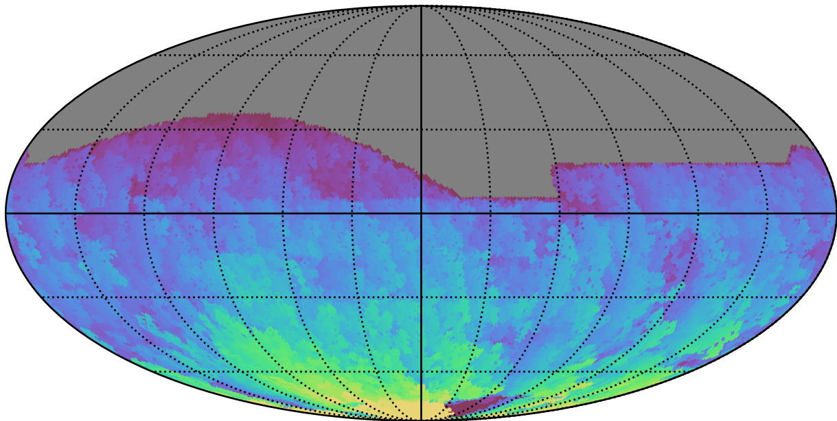
ddf_acor_sf15_lsf40_lsr10_v3.4_10yrs All sky r band: Max HA
